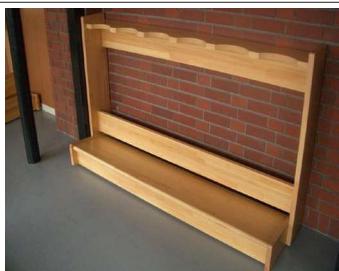
GOY-50 W:1800mm D:450mm H:950mm
